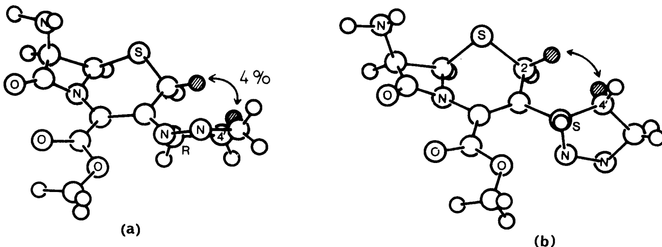
Figure 2. The possible C-3 R (a) and S (b) configurations of compound 4, resulted from the \beta and \alpha face attack of \text{CH}_2\text{N}_2 . The most important nOe value is also shown. For clarity, the 7-acylamido side-chain and the benzhydryl moiety of 4-ester group are omitted.
