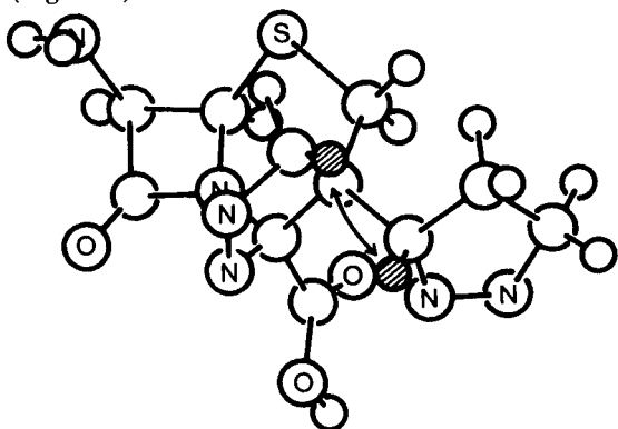
Figure 4. Computer aided design of the structure of the pyrazolinopyrazolilcepham ( 5 ), which corresponds to the observed nOe between 3' H and 5''- H exo .
